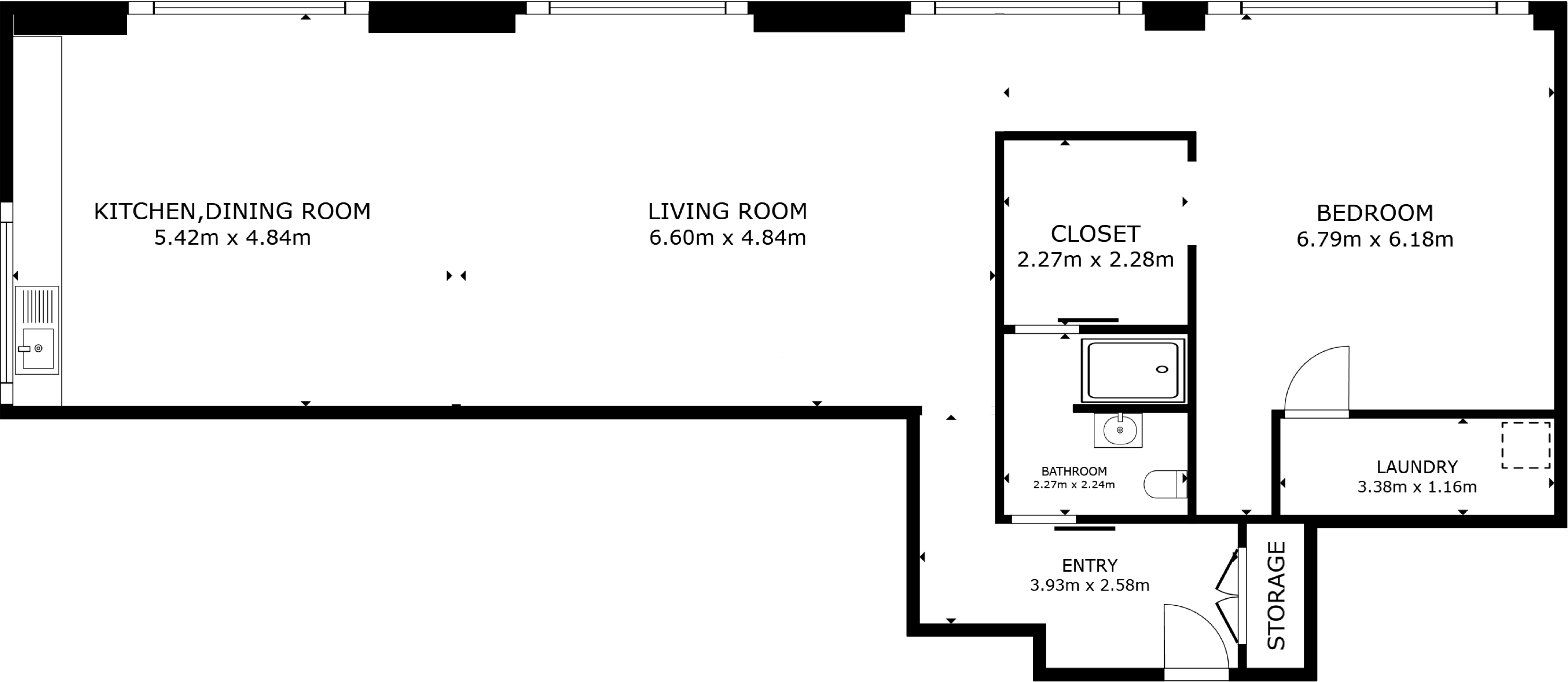
FLOOR PLAN
